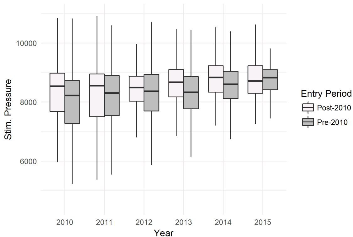
Figure 20: Fracture Pressure by Entrant Date
