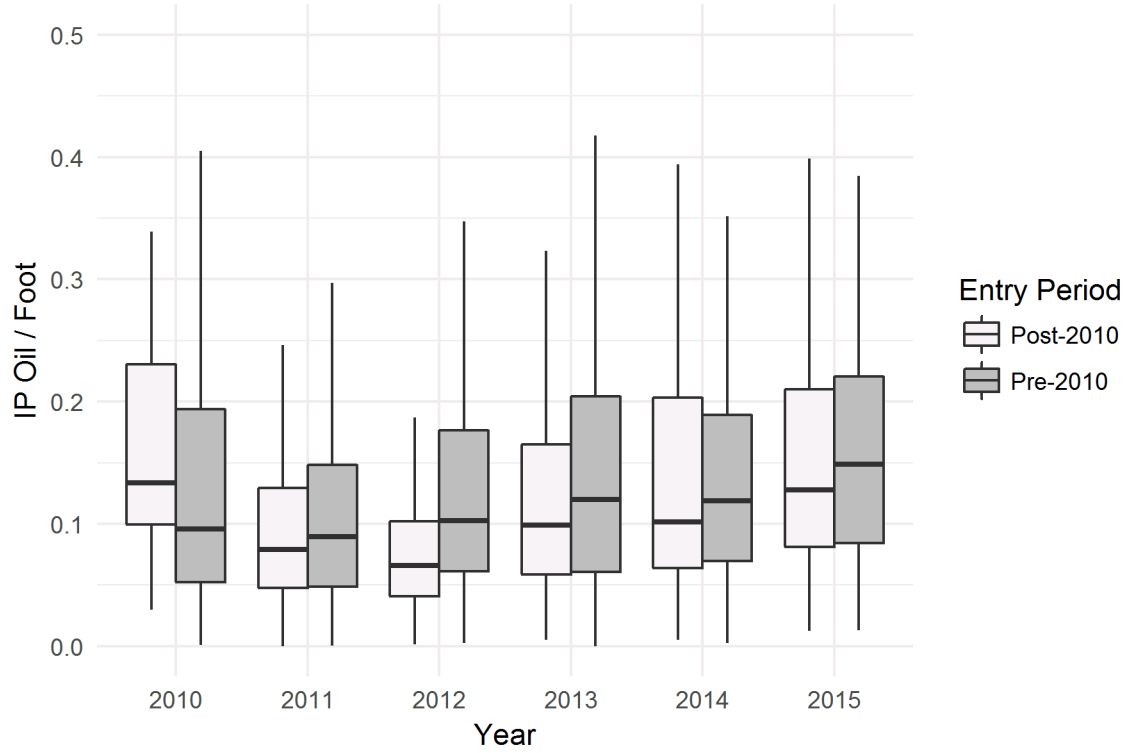
Figure 22: Initial Production per Foot by Entrant Date
