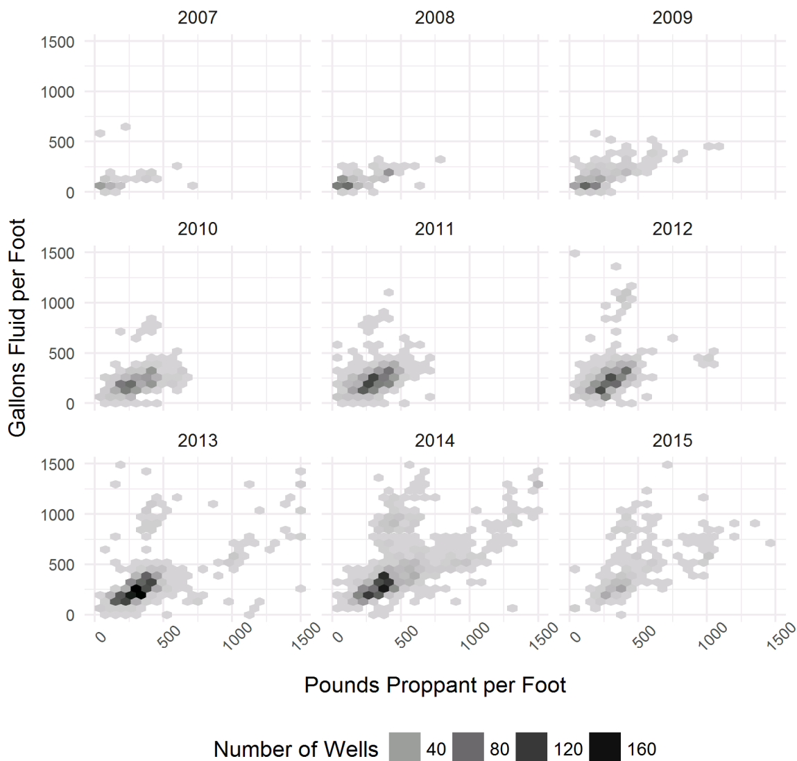
Figure 3: Proppant and Fluid Use, by Year
