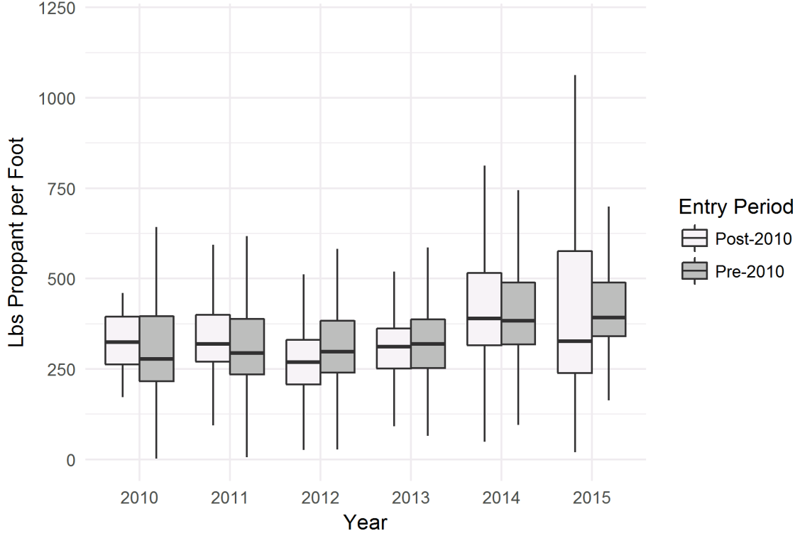
Figure 21: Pounds Proppant per Foot by Entrant Date
